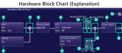
Hardware Block Chart Screen
